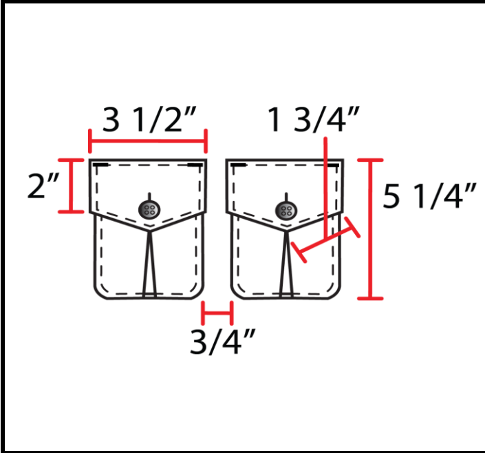
CONSTRUCTION DETAIL NUMBER & DESCRIPTION: Front cargo pockets
