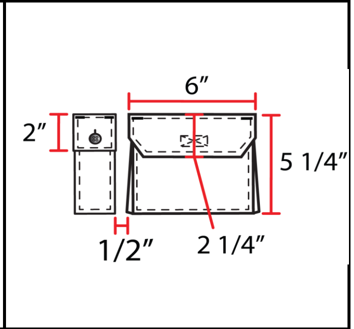
CONSTRUCTION DETAIL NUMBER & DESCRIPTION: Large and small front cargo pocket
