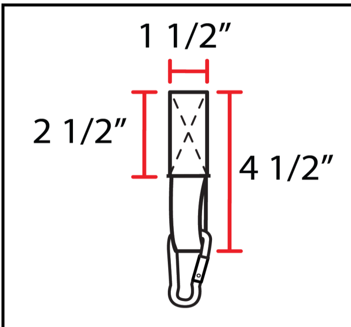
CONSTRUCTION DETAIL NUMBER & DESCRIPTION: Carabiner loop
