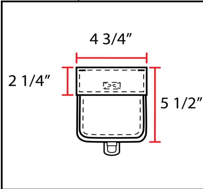
CONSTRUCTION DETAIL NUMBER & DESCRIPTION: Front cargo pocket with D-Rings
