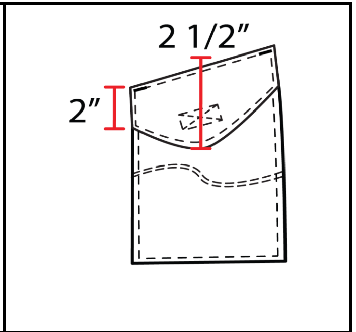
CONSTRUCTION DETAIL NUMBER & DESCRIPTION: Back pocket flaps
